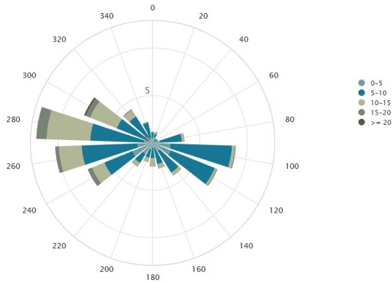
Figure 9: Wind directions.
